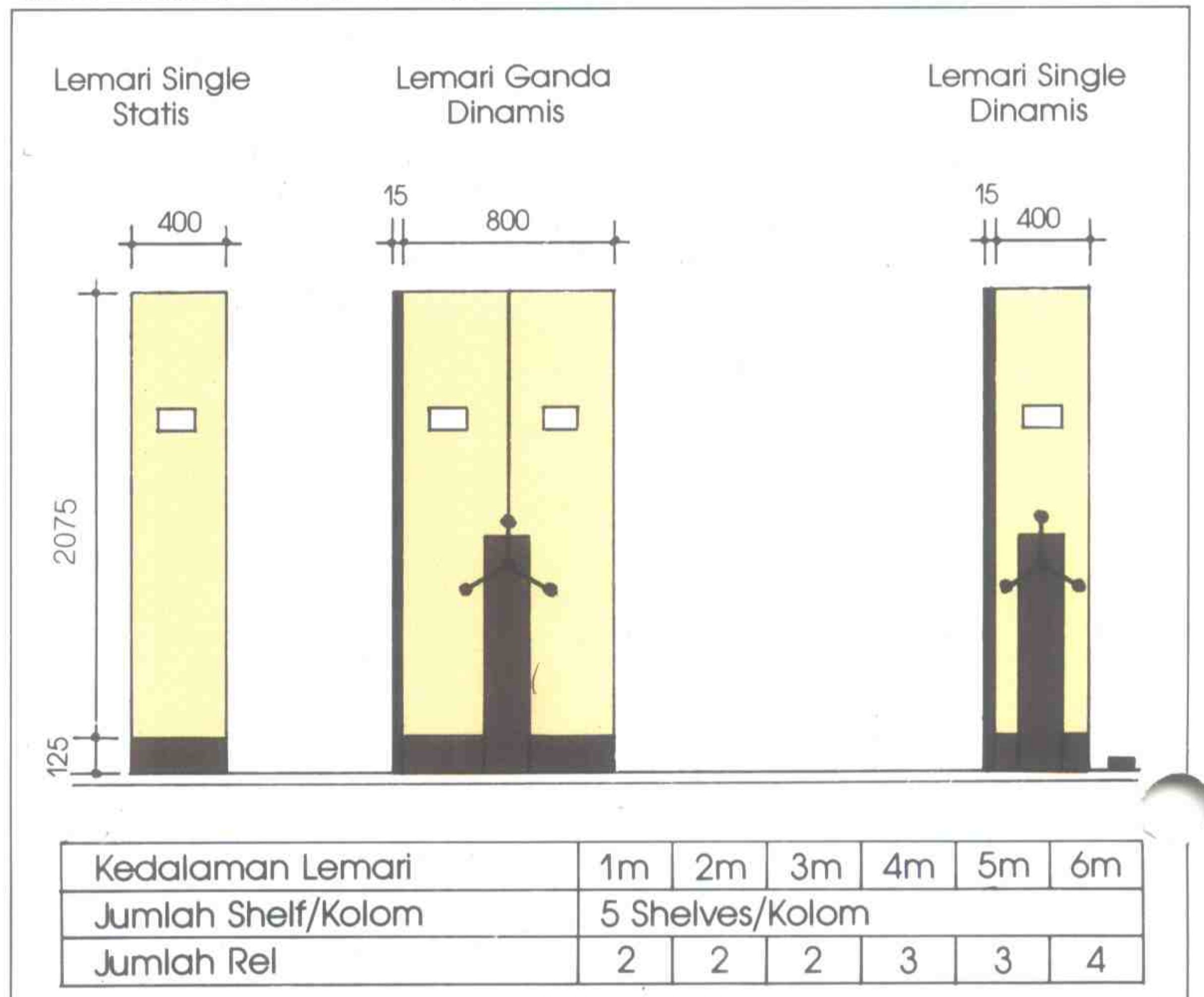
Ukuran Standar Lemari Dorong LION
